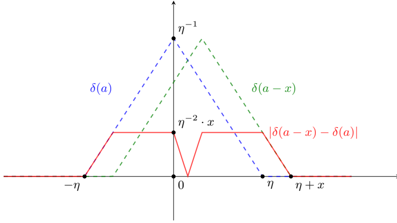
Fig. 1. The surface of |\delta(a - x) - \delta(a)| can be upper bounded by the surface of the isosceles trapezoid with base length 2\eta + x and top length 2\eta - x and height \eta^{-2} \cdot x . This surface equals 2\eta \cdot x .
